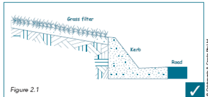
Maintain grassed areas to reduce erosion
