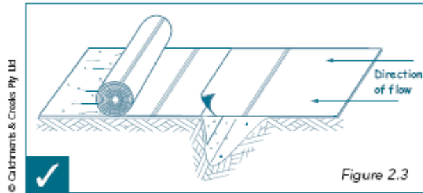
Erosion control blankets can minimise soil erosion
